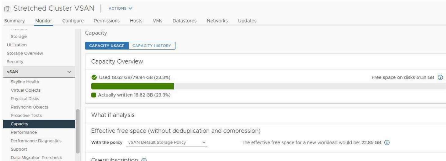
Figura 1: VSAN 7 Capacity
